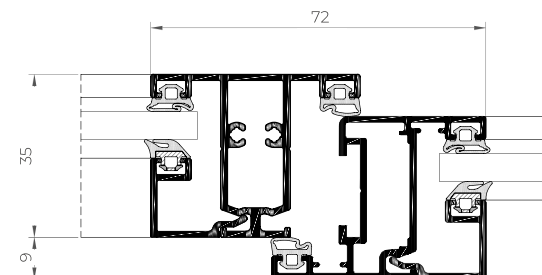
SIDE SASH
