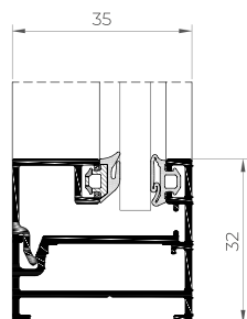
FIXED FRAME
