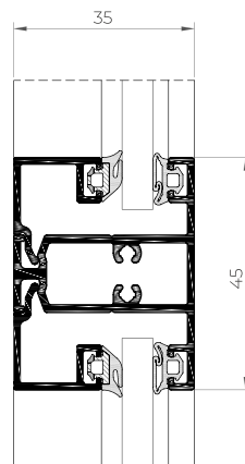
FIXED LIGHT DIVIDER
