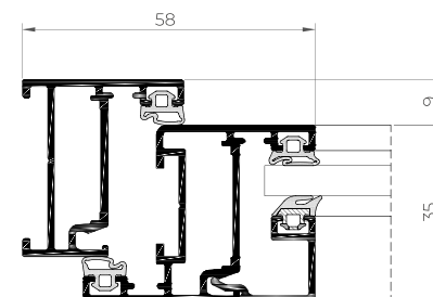
LATERAL SECTION
