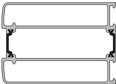
KAS7502 100mm Slave Stile
