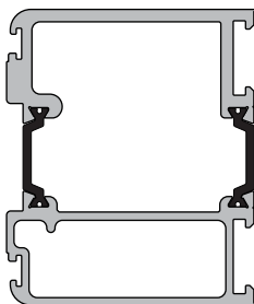
KAS765 Concealed Vertical Rod Stile
