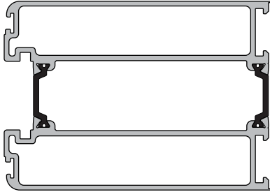
KAS7501 100mm Lock Stile
