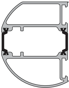
KAS753 Flat Safety Stile
