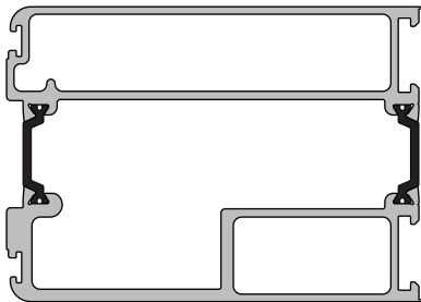
KAS7503 100mm Concealed Vertical Rod Stile
