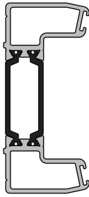
KAS751 Safety Stile Frame
