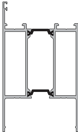
KAS763 Bottom Rail
