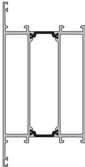
KAS764 Mid Rail
