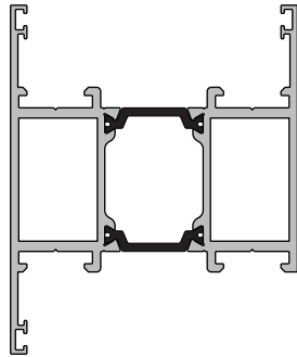
KAS762 Top Rail
